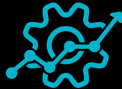
Program Editor
